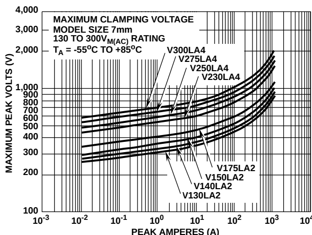
FIGURE 4. CLAMPING VOLTAGE FOR V130LA2 - V300LA4
