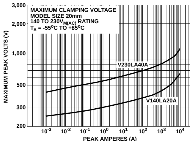
FIGURE 12. CLAMPING VOLTAGE FOR V140LA20A - V230LA40A
