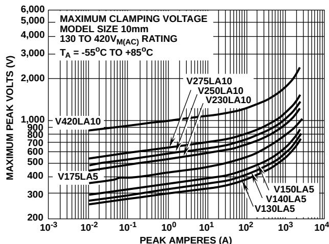
FIGURE 6. CLAMPING VOLTAGE FOR V130LA5 - V420LA10
