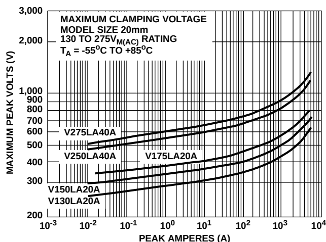
FIGURE 10. CLAMPING VOLTAGE FOR V130LA20A - V275LA40A
