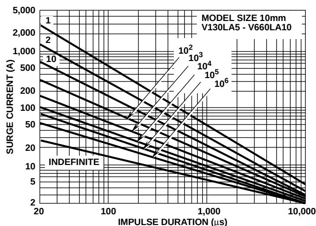
FIGURE 15. SURGE CURRENT RATING CURVES FOR V130LA5 - V660LA10
