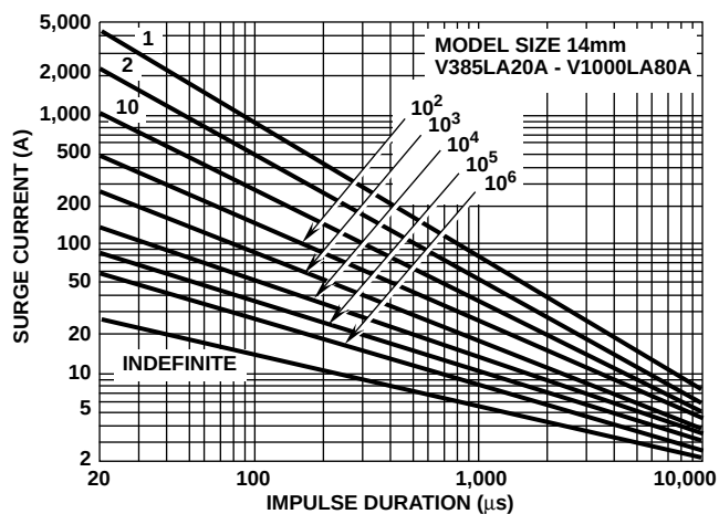
FIGURE 17. SURGE CURRENT RATING CURVES FOR V385LA20A - V1000LA80A
