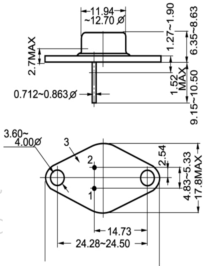
Fig.2 outline dimensions
