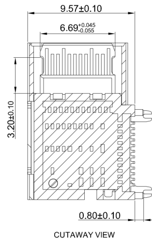
CUTAWAY VIEW
