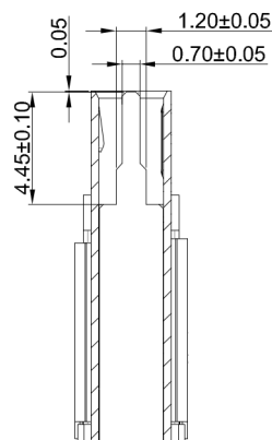
CUTAWAY VIEW
