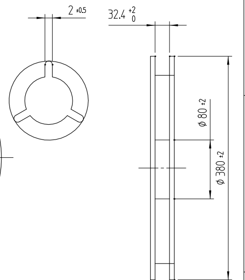
Detail G
