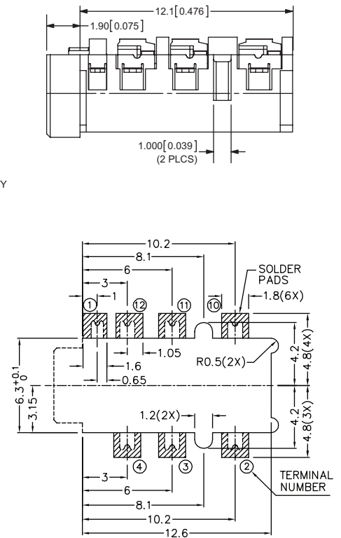
Recommended PCB Layout Top View
