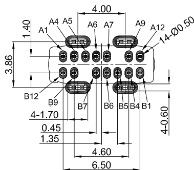
RECOMMENDED P.C.B. LAYOUT TOLERANCE UNSPECIFIED ±0.05mm
