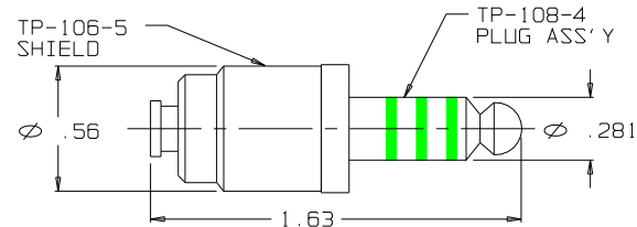
B2 TP-108-6 PLUG & SHIELD ASSEMBLY
