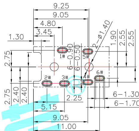
P.C.B. LAYOUT=1.00mm TOP VIEW
