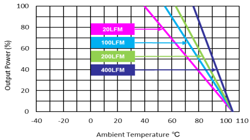
MKWI40-24D12, MKWI40-24D15, MKWI40-48D12, MKWI40-48D15 Derating Curve without Heatsink
