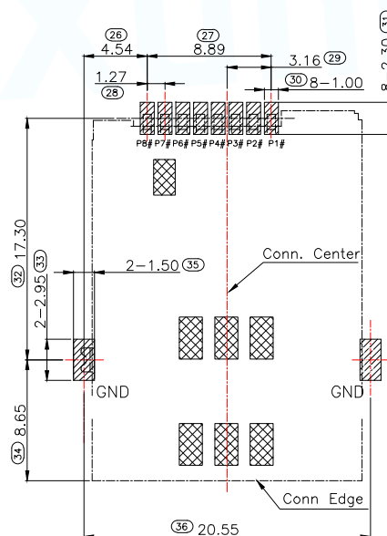
RECOMMENDED PCB LAYOUT(TOP VIEW) GENERAL TOLERANCES:±0.05
