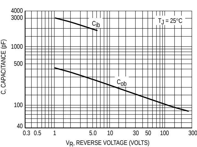
Figure 2. Capacitances
