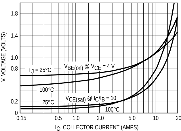
Figure 5. "On" Voltage
