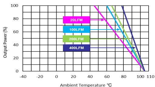
MKW40-XXS05, MKW40-XXS12, MKW40-XXS15, MKW40-XXS24 Derating Curve without Heatsink
