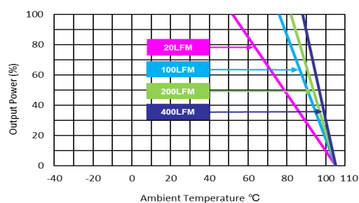
MKW40-XXDXX Derating Curve with Heatsink
